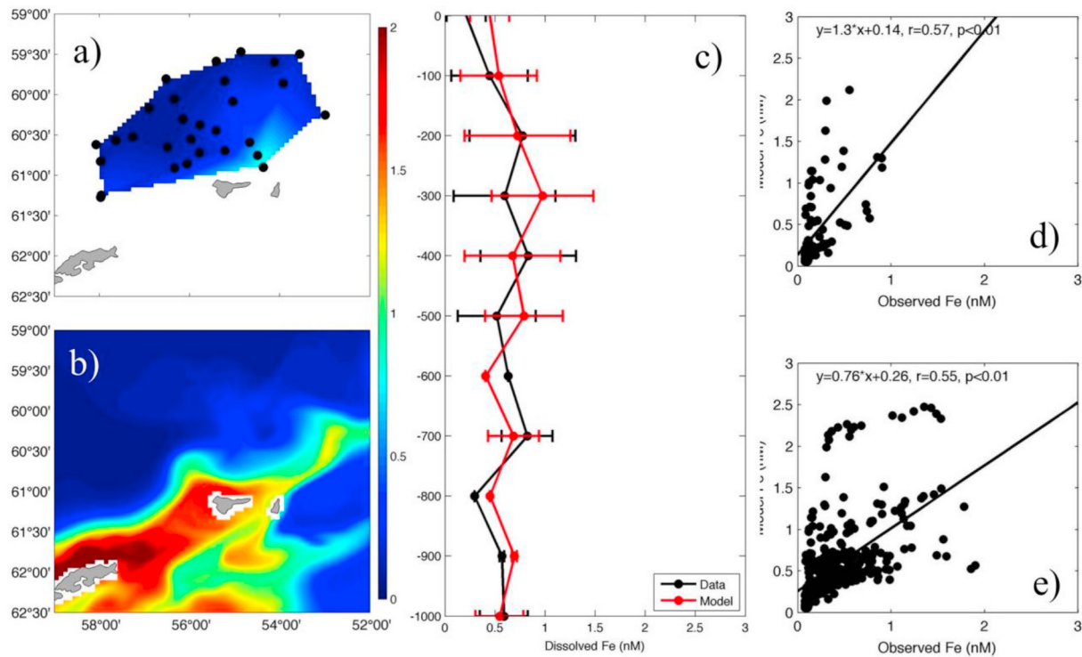
Fig. 7. Surface Fe concentrations from (a) field measurement and (b) model, (c) vertical mean profiles and standard deviation of Fe concentration, and the point-to-point correlation between model and measured Fe concentrations for (d) the surface and (e) all depths during the LMG0402 cruise (Feb–Mar. 2004).
