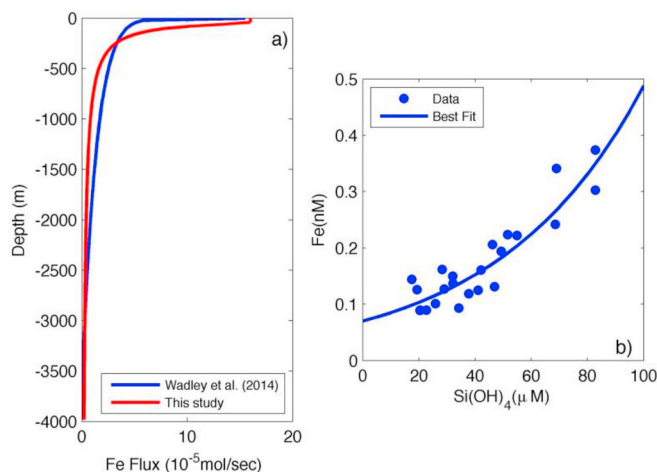
Fig. 3. (a) Sediment Fe flux (mol/sec) in this study (red) and that used by Wadley et al. (2014) (blue), and (b) Fe concentration (nM) versus \text{Si(OH)}_4 concentration ( \mu\text{M} ) at two stations representing the ACC waters during the summer (LGM0402) cruise. The blue line represents the best exponential fit, y = 0.0701e^{0.0194x} ( r = 0.88 , p < 0.01 ). (For interpretation of the references to color in this figure legend, the reader is referred to the Web version of this article.)
