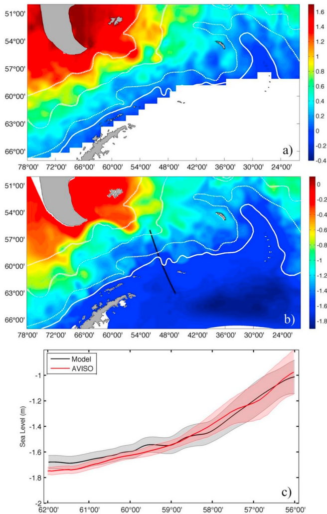
Fig. 4. Monthly mean sea level from (a) AVISO and (b) model during August 2006, and (c) multyear mean and standard deviation (STD) of SSH along a transect (black line in (b)) from the Weddell Sea to Drake Passage. No valid satellite altimetry data exist in the Weddell Sea and much of the AP shelf (blank area) during winter time. White lines indicate the ACC fronts (Orsi et al., 1995).
