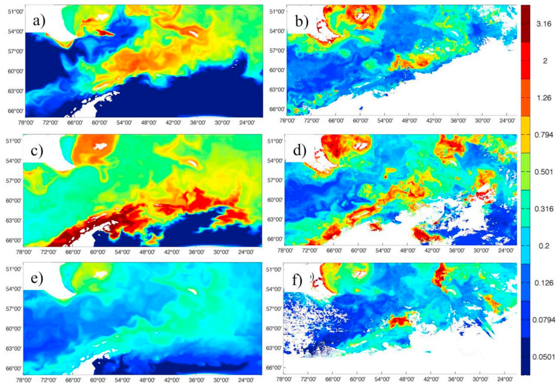
Fig. 9. Monthly means of model surface chlorophyll (a, c, e) and the monthly composites of MODIS surface chlorophyll (b, d, f) for October 2005 (a, b), January 2006 (c, d) and April 2006 (e, f), respectively.
