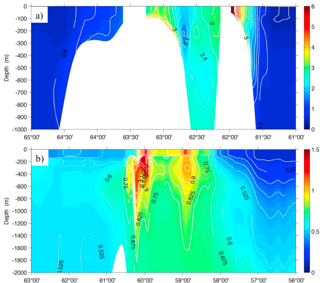
Fig. 11. Vertical distributions of model dissolved Fe concentration during August 2006 along (a) the mid-Bransfield transect (across the Antarctic Sound and King George Island, shown as a black line in Fig. 10) and (b) Weddell-Drake Passage transect (from Powell Basin to Ona Basin, shown as a black line in Fig. 10).
