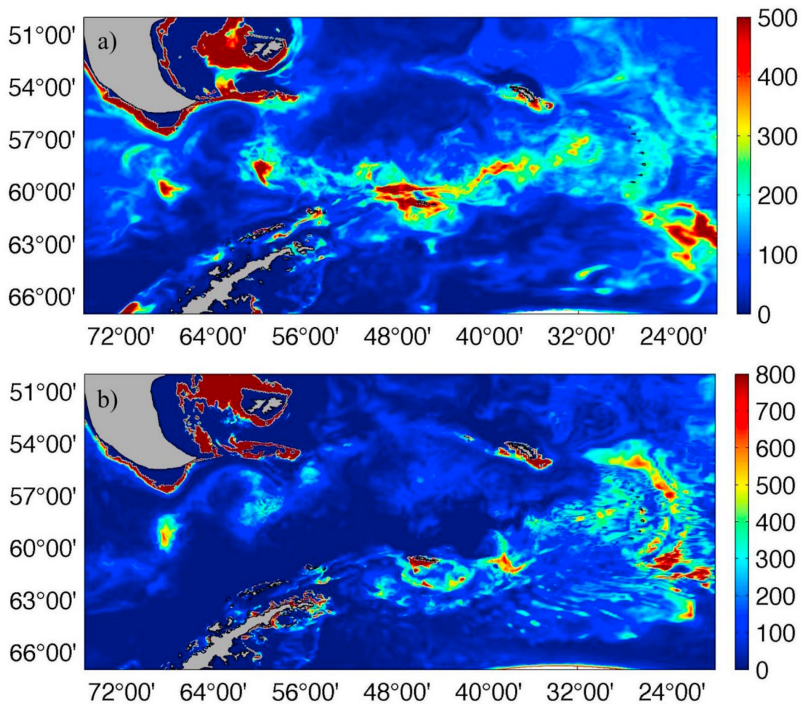
Fig. 16. Multi-year (2003-2006) average of vertical Fe flux ( \mu\text{mol}/\text{m}^2/\text{year} ) at the base of the mixed layer in summer (December-February) (a) and winter (June-August) (b). The base of the mixed layer is defined as 50 m for the summer and 100 m for the winter.
