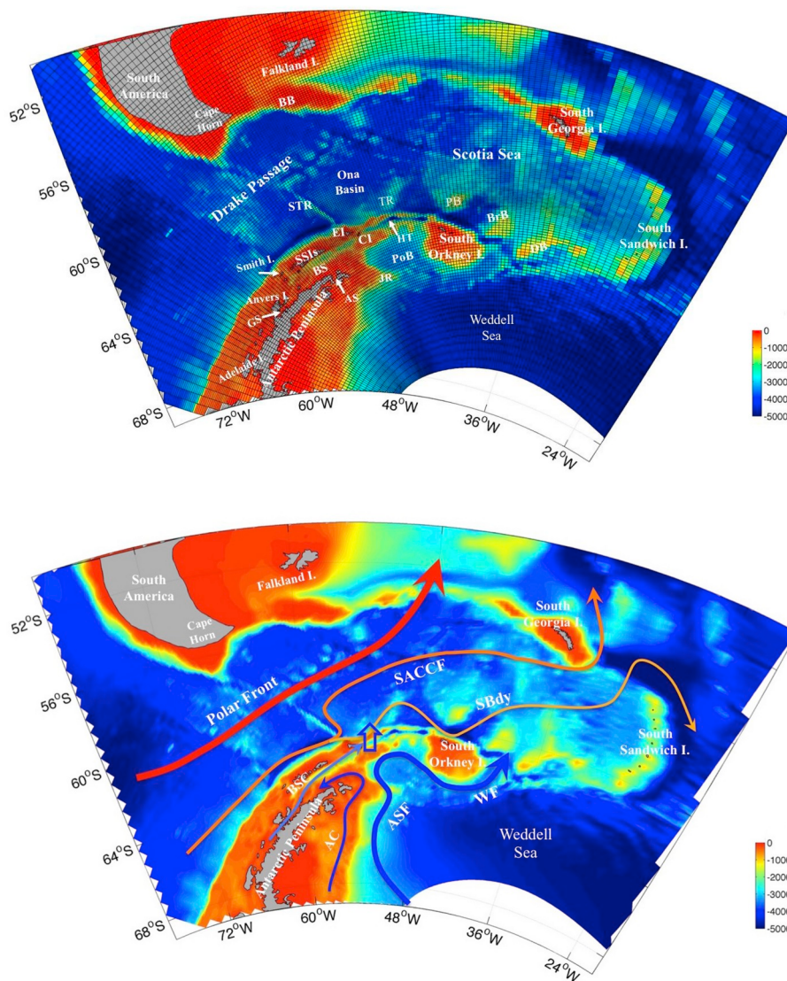
Fig. 1. Top panel: Model grid (sub-sampled 1 per 3 grid lines) and topography for the study area. Acronyms: BB – Burdwood Bank, STR – Shackleton Traverse Ridge, TR – Terror Rise, PB – Pirie Bank, BrB – Bruce Bank, DB – Discovery Bank, SSIs – South Shetland Islands, EI – Elephant Island, CI – Clarence Island, BS – Bransfield Strait, HT – Hesperides Trough, PoB – Powell Basin, GS – Gerlache Strait, AS – Antarctic Sound, JR – Joinville Ridge. Bottom panel: Diagram of major currents in the study area. Acronyms: SACCF – Southern ACC Front, SBdy – Southern ACC Boundary, BSC – Bransfield Straits Current, ASF – Antarctic Slope Front, AC – Antarctic Coastal Current, WF – Weddell Front. Broad open arrow indicates the off-shelf export. We do not distinguish between the SACCF and the SBdy west of the Shackleton Traverse Ridge.
