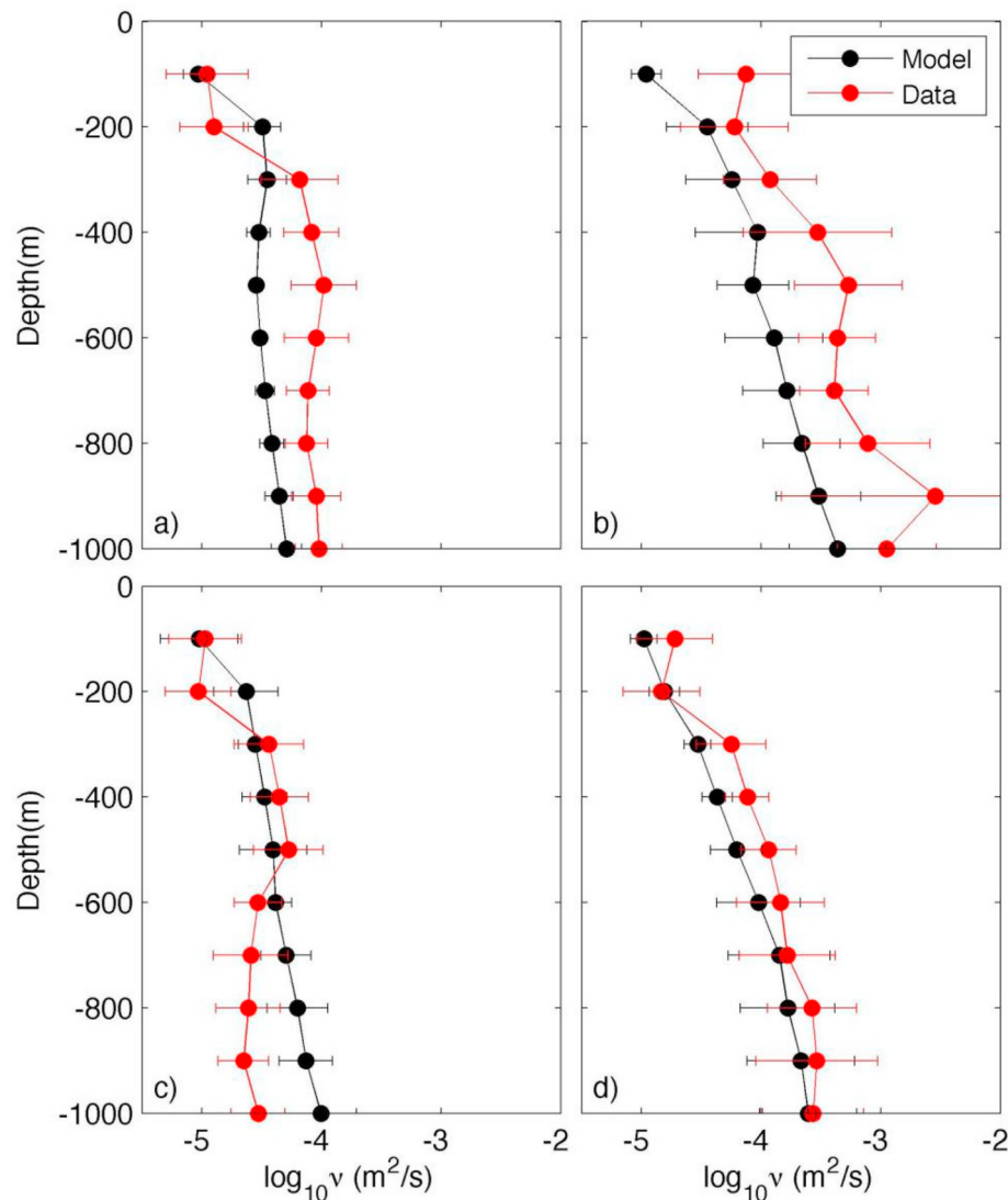
Fig. 6. Vertical mixing from estimates based on in situ measurements and model output for (a) Drake Passage, (b) north Scotia Ridge, (c) south Scotia Ridge, and (d) southern Scotia Sea. The in situ estimates were derived from Naveira Garabato et al., (2004). Model output is from summer (February) 2006.
