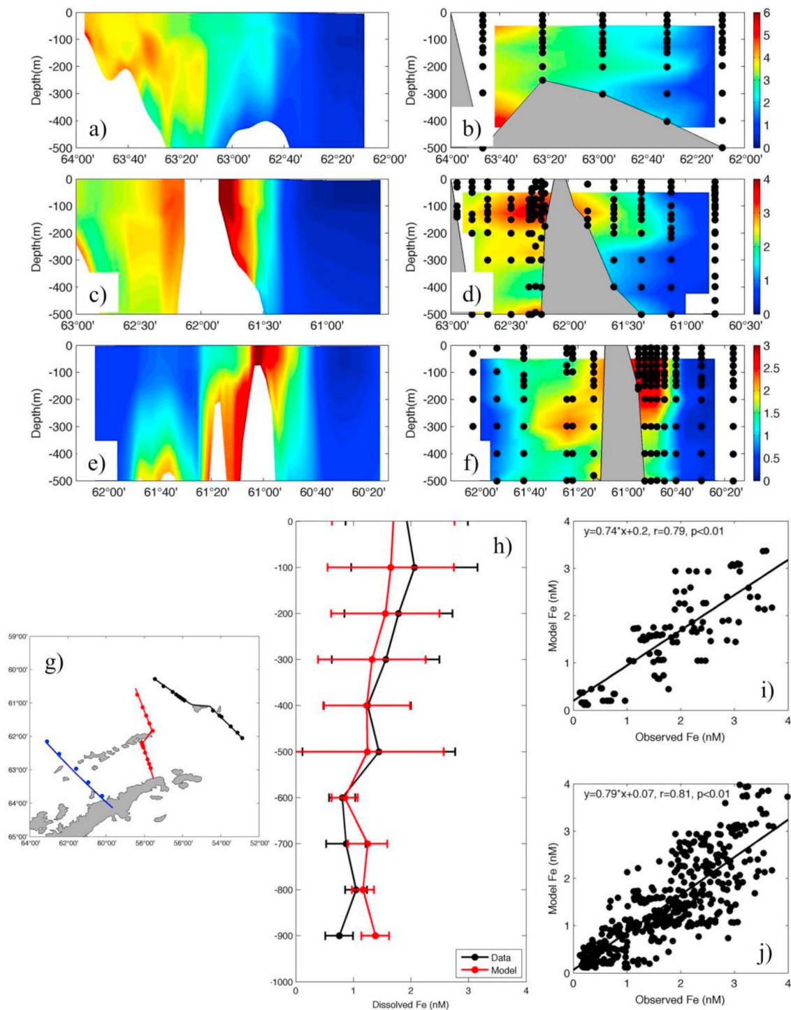
Fig. 8. (a–f) Modeled (a, c, e) and field measured Fe concentrations (b, d, f) during the NBP0606 cruise along the three transects across the Bransfield Strait. (g) The model transects (solid lines) and stations (dots) (blue line: a & b; red line: c & d; black line: e & f). (h) The vertical mean profiles and standard deviation. (i)–(j) the scatter plot of the point-to-point modeled versus data for (i) the surface only and (j) data from all depths (solid lines are the best linear regression between model–data). (For interpretation of the references to color in this figure legend, the reader is referred to the Web version of this article.)
