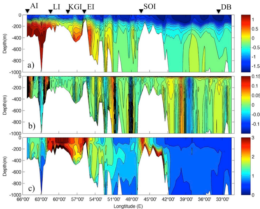
Fig. 14. (a) Vertical distributions of (a) temperature ( ^{\circ}\text{C} ), (b) cross-section velocity (m/sec) (northward positive), and (c) dissolved Fe concentration (nM) along the shelf edge transect (see red dotted line in Fig. 10). Acronyms: AI – Anvers Island, LI – Livingston Island, KGI – King George Island, SOI – South Orkney Island, DB – Discovery Bank. (For interpretation of the references to color in this figure legend, the reader is referred to the Web version of this article.)
