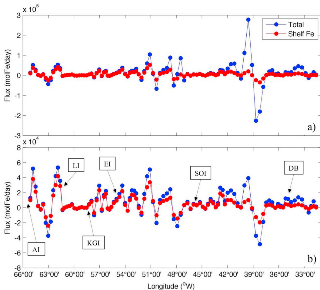
Fig. 15. Depth-integrated off-shelf transport flux of dissolved Fe (mol/day) in the entire water column (a) and the upper 500 m (b) for total (blue dots) and shelf-derived Fe only (red dots) along the AI-EI-SOI-DB transect. The flux is computed at 15 km increment. For acronyms, see Fig. 14. (For interpretation of the references to color in this figure legend, the reader is referred to the Web version of this article.)
