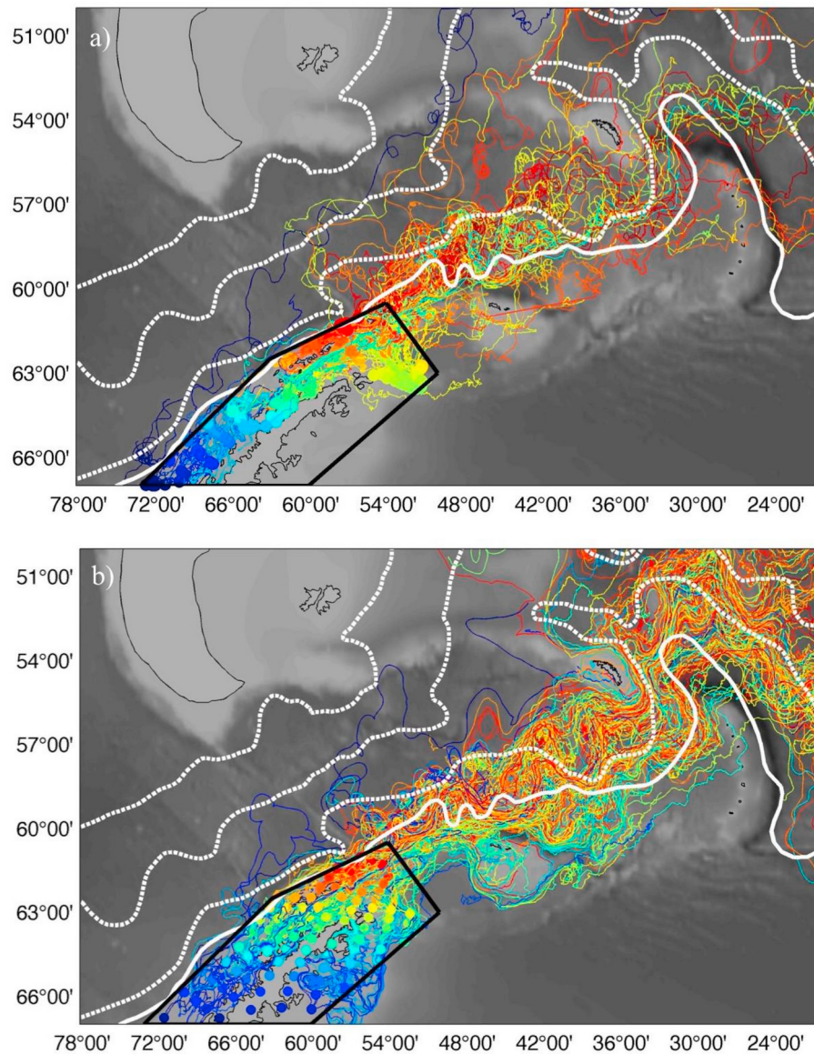
Fig. 5. Trajectories of surface drifters (a) (data source: https://gdp.aoml.gov/ ) and model neutrally buoyant particles (b) released from the AP shelf. Modeled particles were uniformly seeded over the AP waters (inside the black box with dots indicating the initial positions) and continuously released for 2 months starting June 1, 2006. White dashed and solid lines indicate the ACC fronts and SBdy, respectively.
