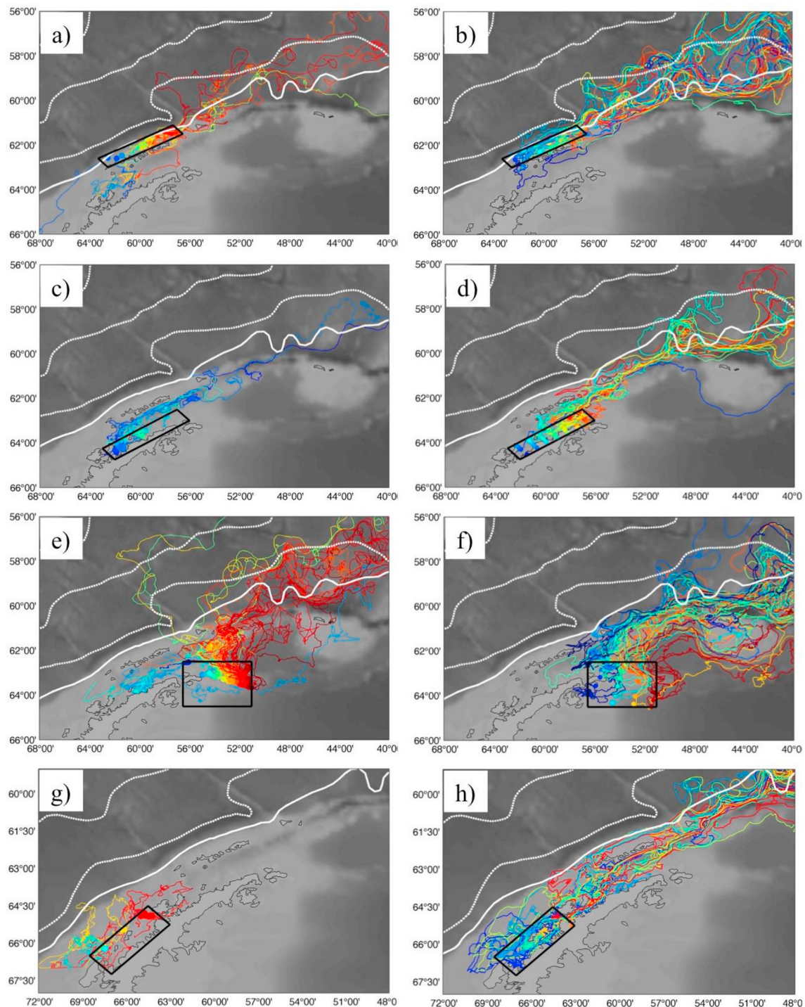
Fig. 13. Trajectories of surface drifters (left panels) and modeled particles (right panels). The black box shows the release area: the northern SSIs shelf (a, b), the southern Bransfield Strait shelf (c, d), the northwest Weddell Sea (e, f) and the western Antarctic Peninsula shelf (g, h). Colored dots indicate the initial positions of the particles/drifters.
