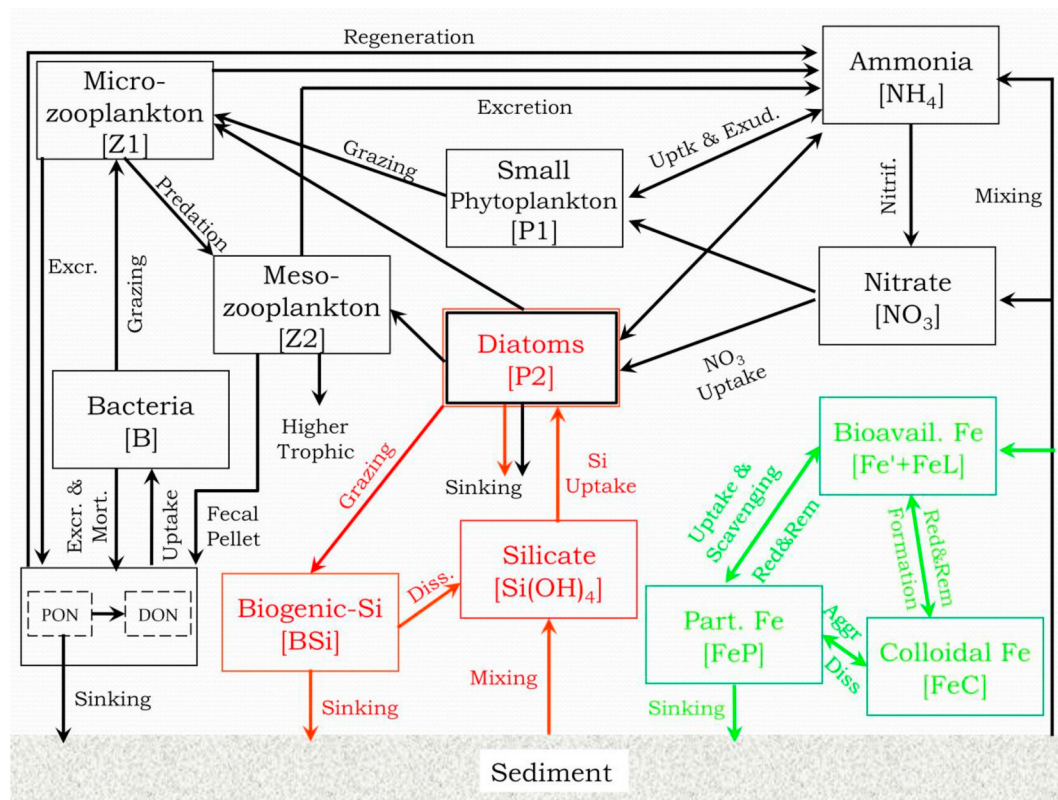
Fig. 2. Diagram of the biogeochemical model (SOFe) (reproduced from Jiang et al., 2013a). Color codes are for nitrogen (black), silica (red), and Fe (green) flows, respectively. For clarity some minor elemental flows were not included. No sediment sub-model is incorporated in the current study. Bio-available Fe includes both dissolved inorganic Fe ( \text{Fe}' ) and Fe bound to organic ligands ( \text{FeL} ). PON and DON represent, respectively, particulate and dissolved organic nitrogen. More details of the model can be found in Jiang et al. (2013a). (For interpretation of the references to color in this figure legend, the reader is referred to the Web version of this article.)
