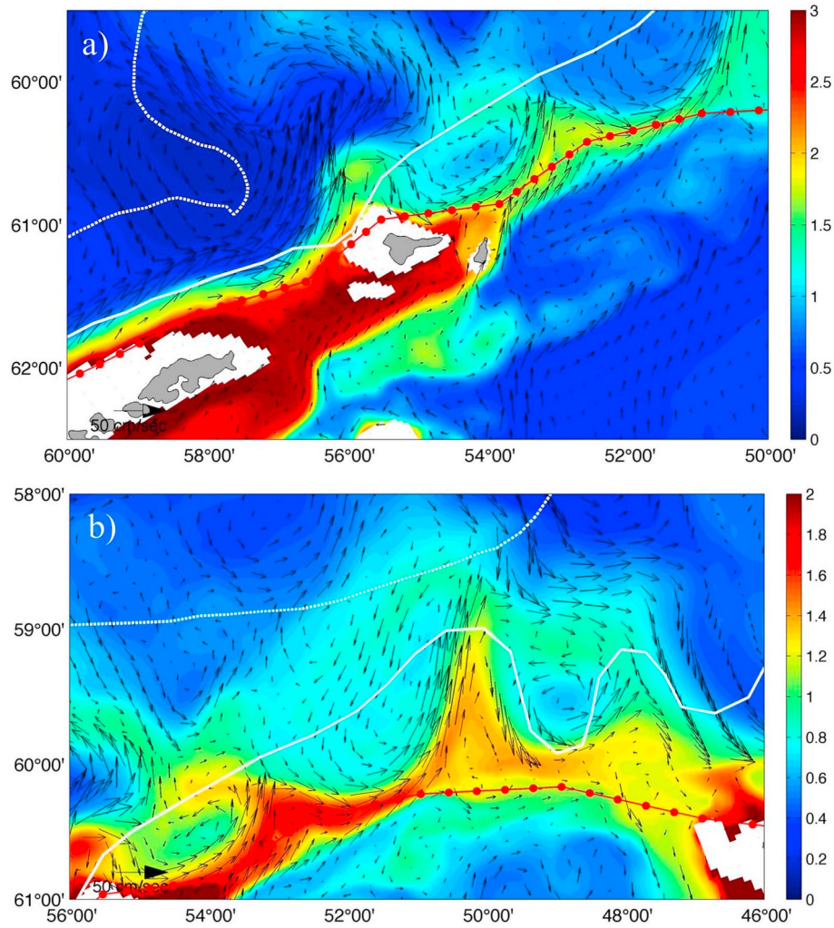
Fig. 12. Horizontal distributions of modeled dissolved Fe concentration (color) and currents (arrows) at 200 m in August 2006 for the Elephant Island area (a) and around Terror Rise (b). White dashed and solid lines indicate the ACC fronts (PF and SACCF) and SBdy fronts, respectively. Red dotted line indicates the portions of along-shelf transect in Fig. 10. (For interpretation of the references to color in this figure legend, the reader is referred to the Web version of this article.)
