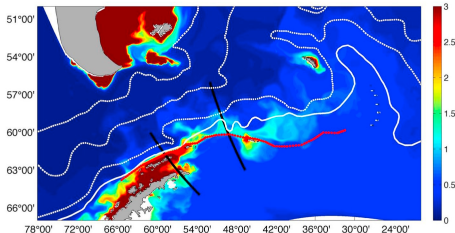
Fig. 10. Horizontal distributions of modeled surface dissolved Fe in August 2006. The black lines indicate the two N-S south transects: mid-Bransfield transect (across the Antarctic Sound and King George Island), and Weddell-Drake Passage (from Powell Basin to Ona Basin), respectively. The red dotted line indicates the along-shelf transect from Adelaide Island to Elephant Island, SOI and Discovery Bank (AI-EI-SOI-DB) for estimates of cross-shelf Fe transport shown in Fig. 14 and 15. White lines indicate the ACC fronts (from north to south): SAF, PF, SACCF, and SBdy. (For interpretation of the references to color in this figure legend, the reader is referred to the Web version of this article.)
