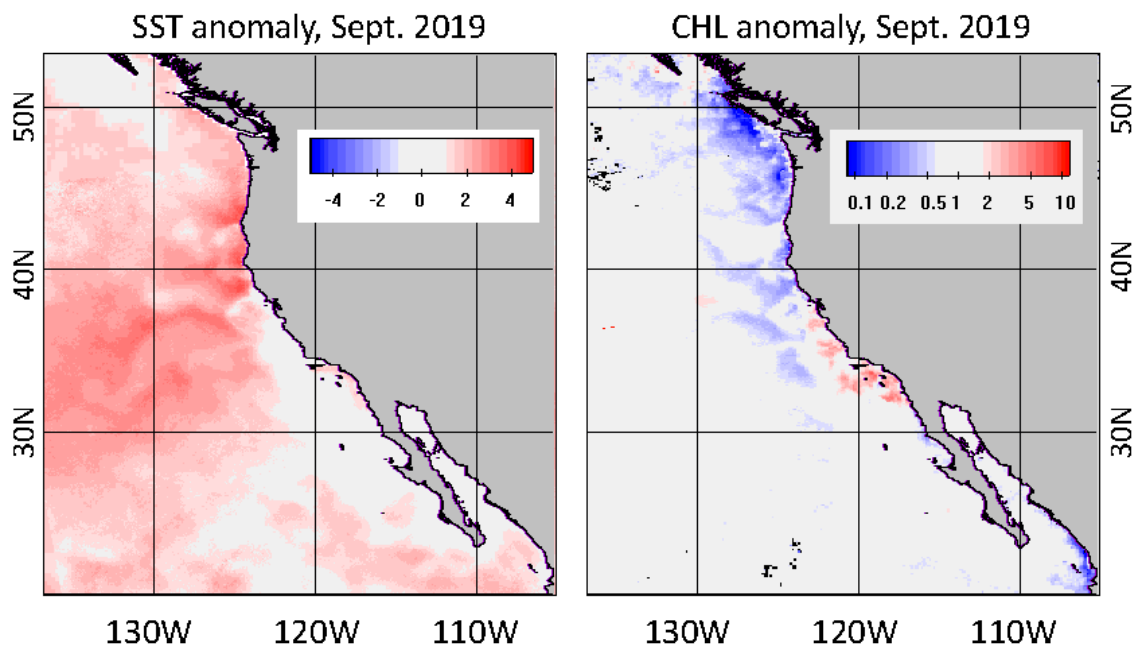
Figure 13. Spatial patterns of September, 2019 anomalies in SST and chlorophyll a . The SST anomaly was computed as difference from the long-term mean (1981–2019) in °C. The chlorophyll a anomaly was expressed as ratio to the long-term mean (1996–2019).
