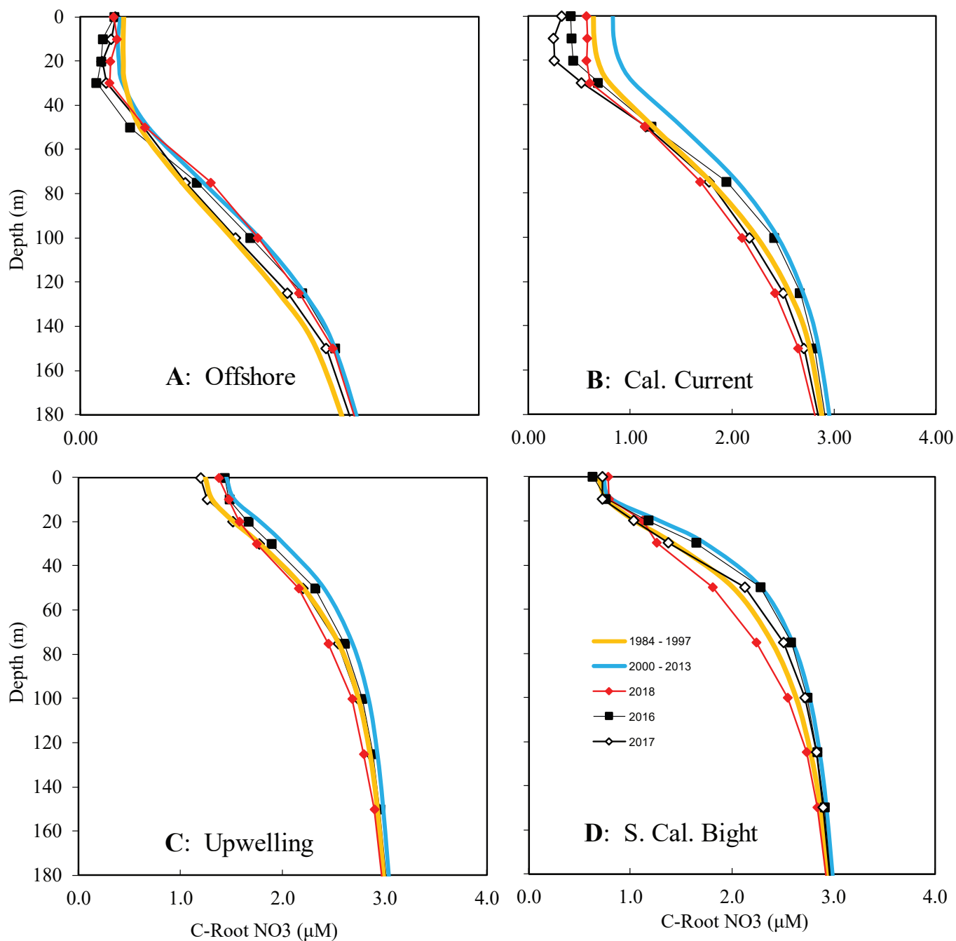
Figure S3. Depth profiles of cuberoot of nitrate for the times and four areas of the CalCOFI region that are defined in CalCOFI Fig. S1. Data were derived and are presented as described in CalCOFI Fig. S1.
