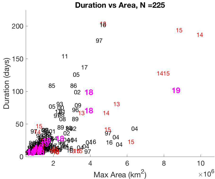
Figure 14. Duration of all marine heat waves (MHW)s >5 days long vs maximum area of each MHW, with the year of the feature initiation labeled. Highlighted are the main “blob” years of 2013–14 in red, and the most recent MHW of 2018 and 2019 in magenta.
